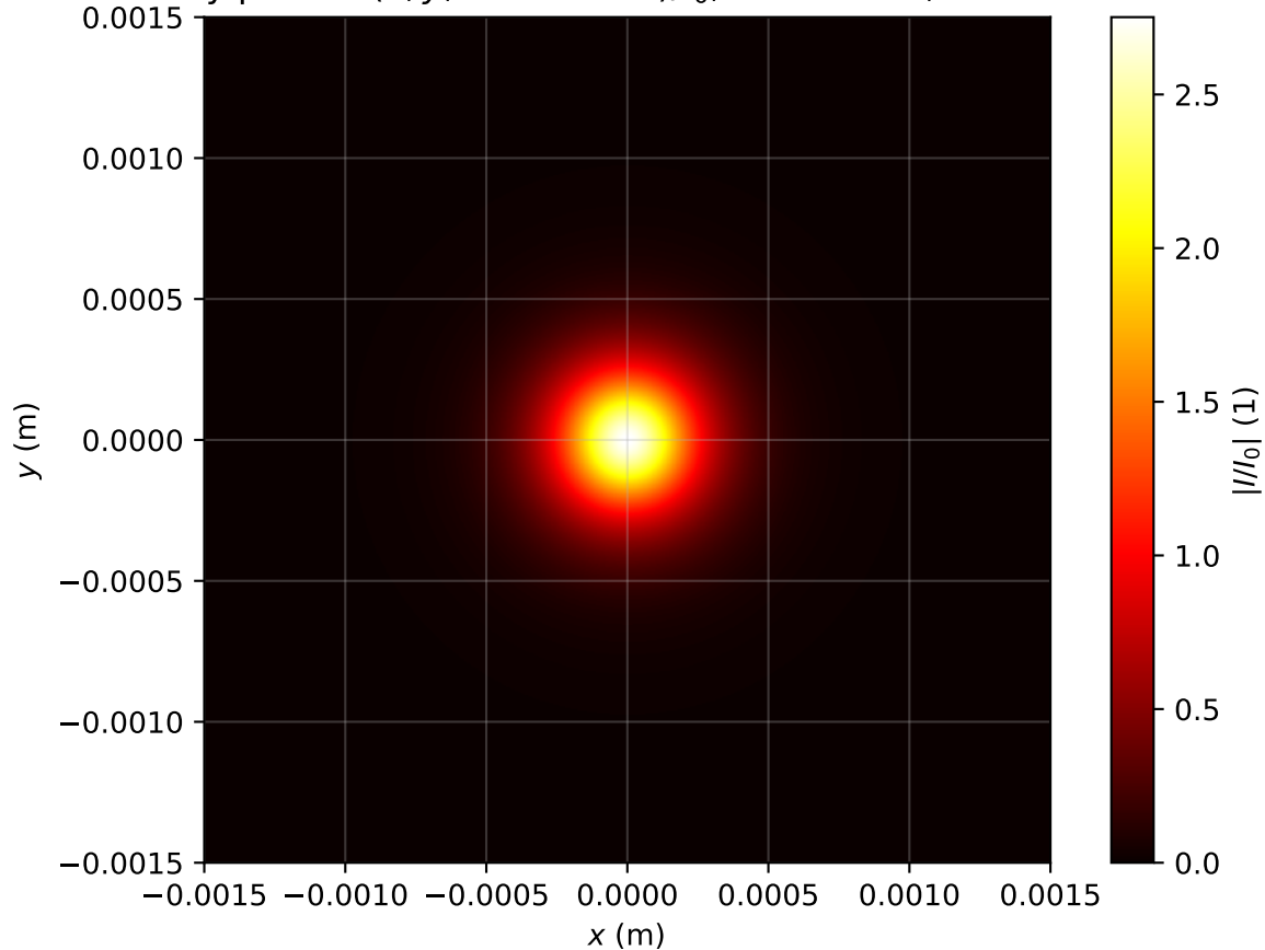
Intensity profile I(x, y, z = 3.184m)/I_0 , P_{in}=1.0P_{cr} , artificial time
